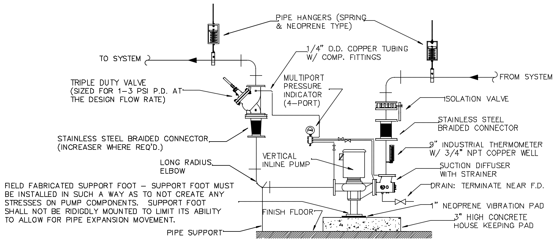
4 VERTICAL INLINE PUMP DETAIL - (FLOOR MOUNTED ON A HOUSEKEEPING PAD) NOT TO SCALE
