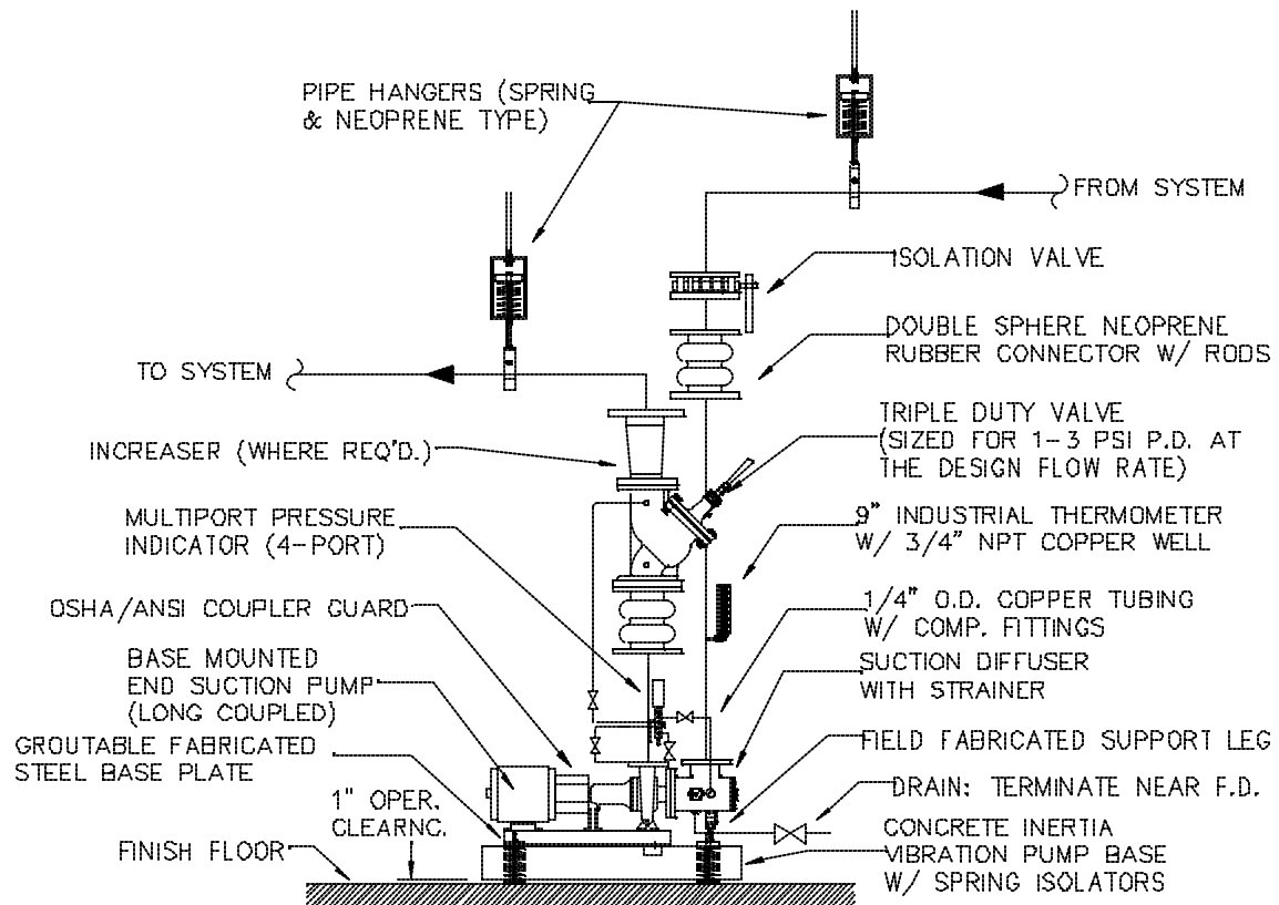
4 END SUCTION PUMP DETAIL - (BASE MOUNTED ON CONCRETE INERTIA BASE) NOT TO SCALE
